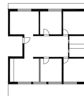
Siedlung Bockler, Zürich, Switzerland. Christoph Haerle & Sabina Hubacher 2007.
