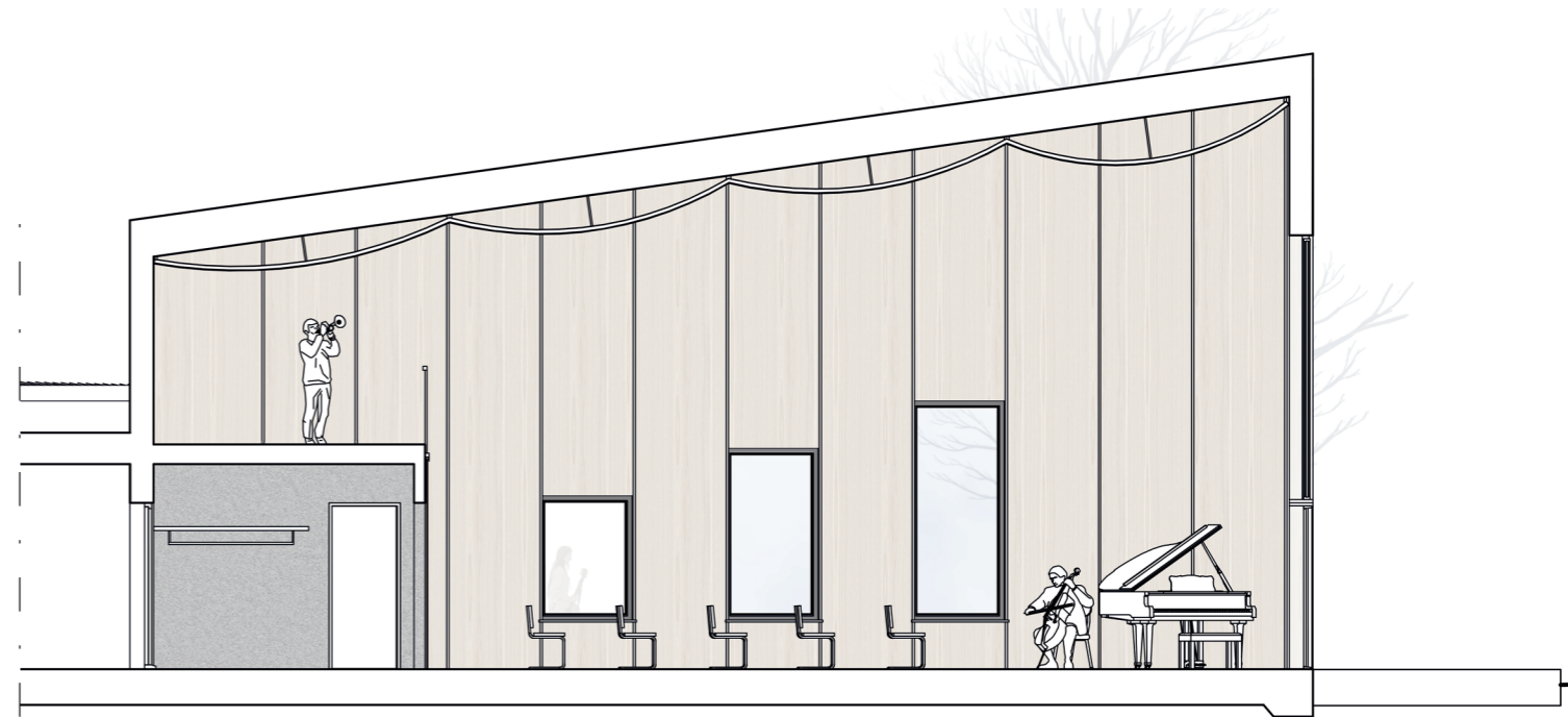
Section D-D, Concert hall
