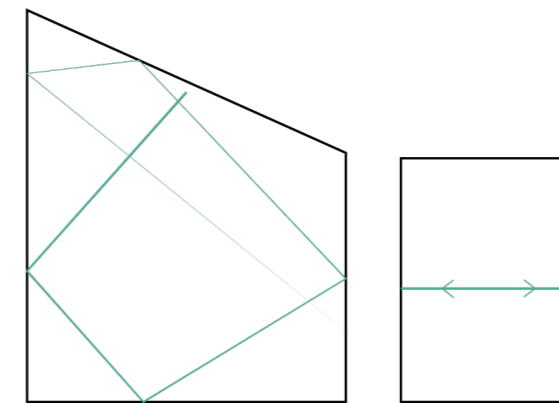
Angled surfaces scatter the sound waves and avoid flutter echoes that distort the soundscape.
