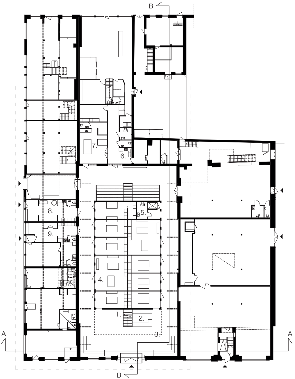
GROUND LEVEL. Scale 1:400.
