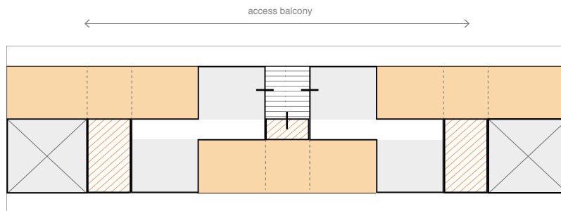
apartment configuration normal plan B 1:400
