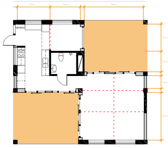
Type 1 measurement plan
