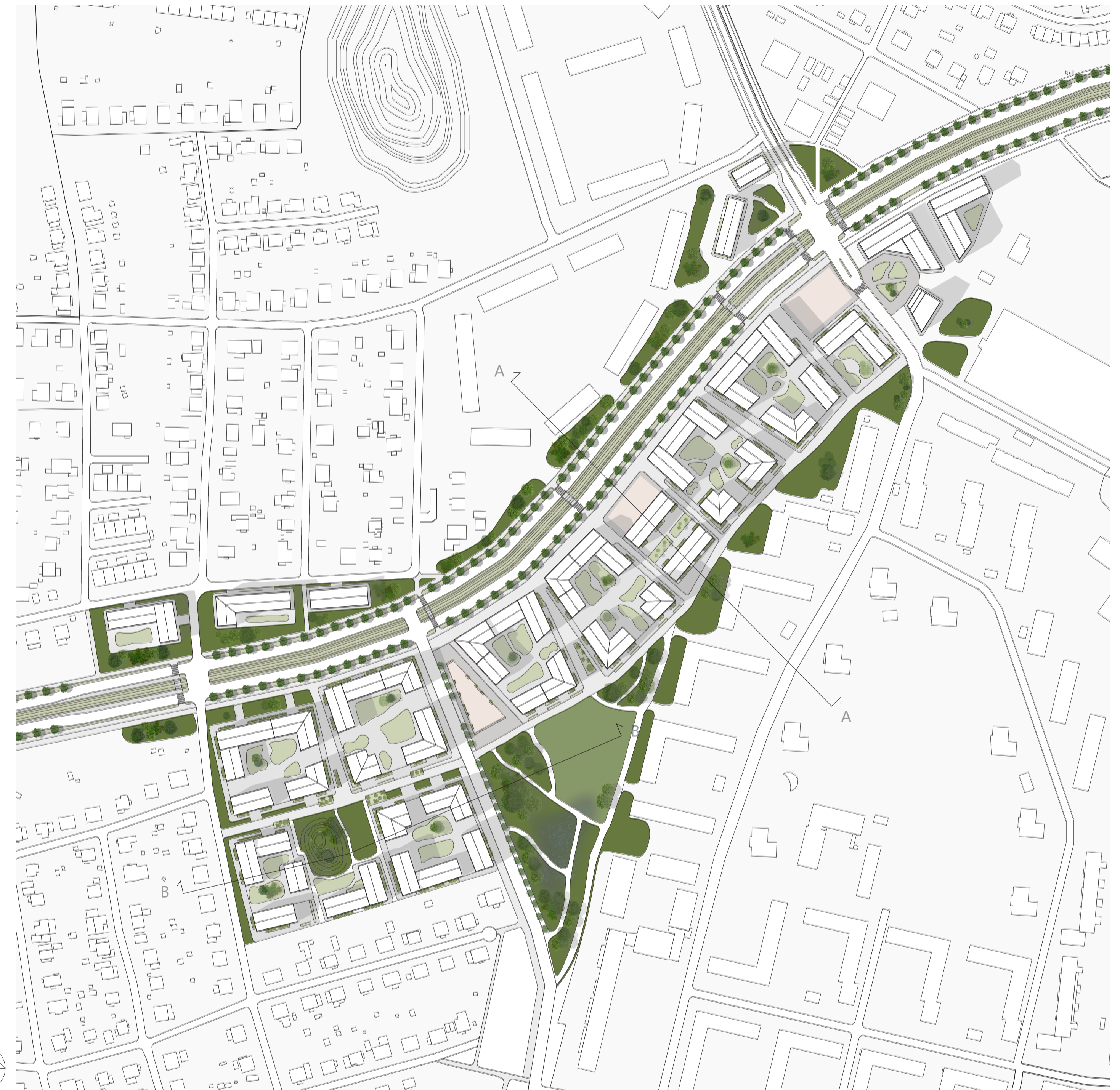
Situationsplan 1:2000 (A1)
